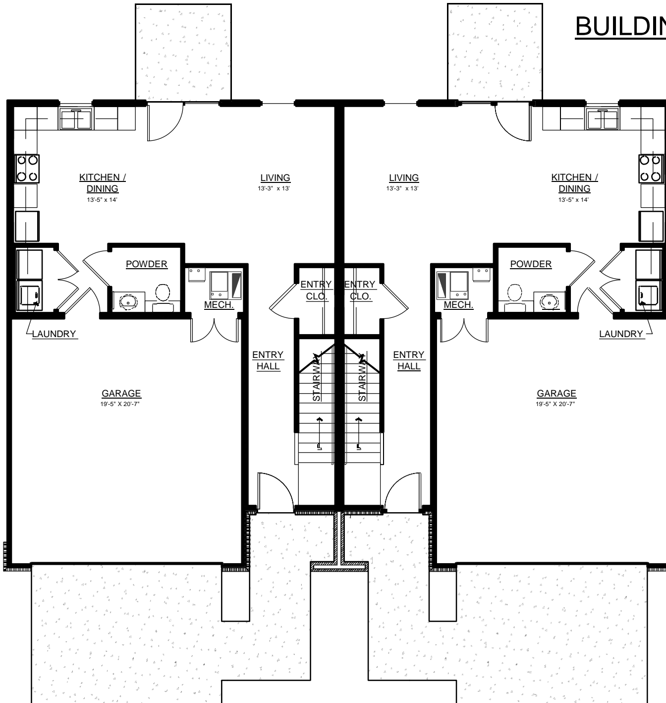
FIRST FLOOR PLAN - 2 BEDROOM / 1.5 BATH DUPLEX
