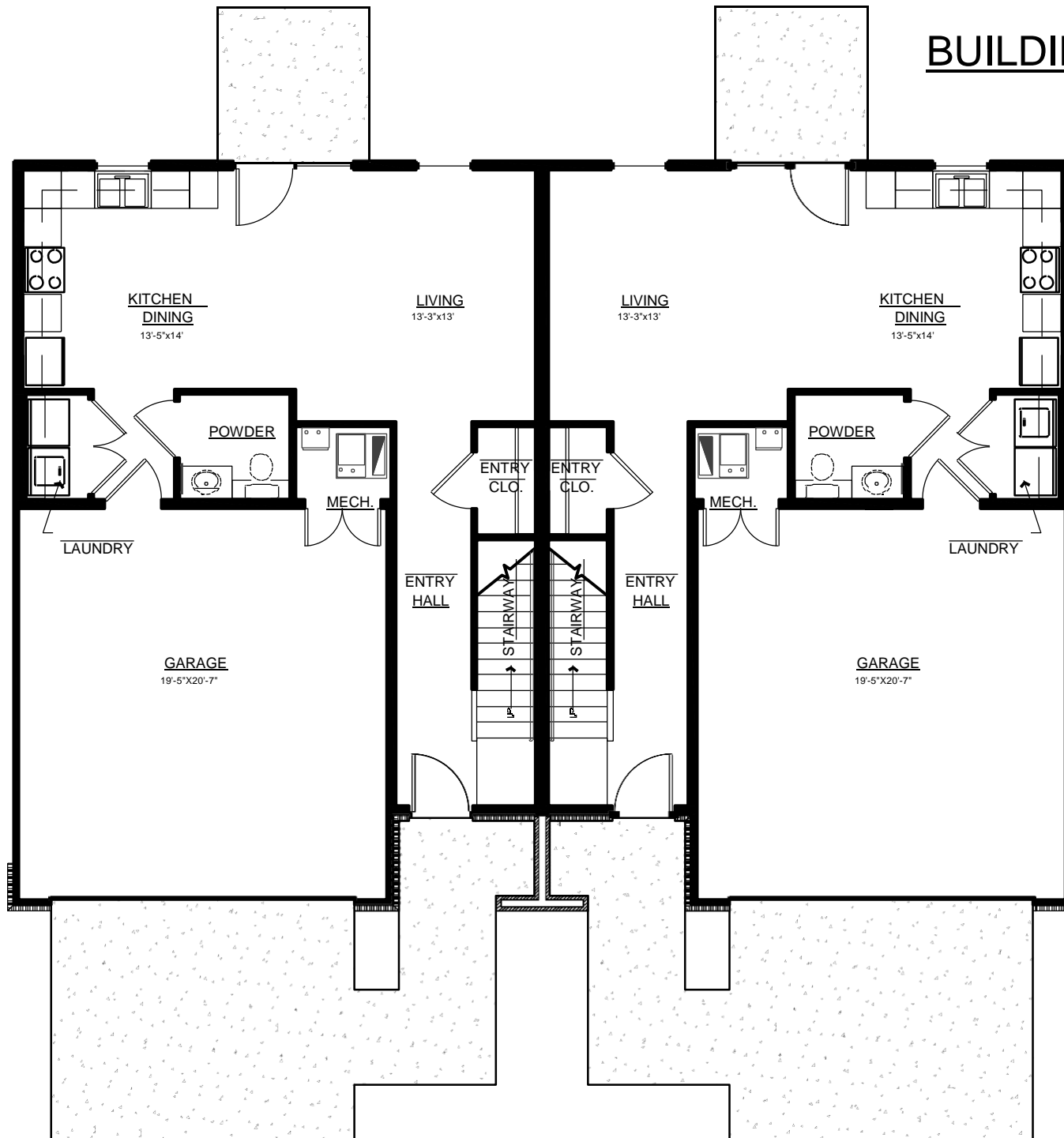
FIRST FLOOR PLAN - 3 BEDROOM 2.5 BATH DUPLEX
